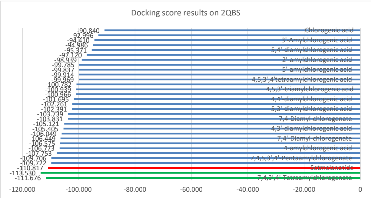
Figure 5. Docking score results on 2QBS; blue line indicates as inactive compound, red line indicate as positive control and green line indicates as the active compound
