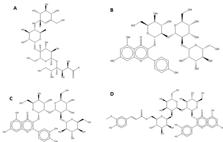
Figure 1. Structure of A) Acarbose B) Kaempferol 3-glucosyl-(1-2)-galactosyl-(1-2)-glucoside ; C) Quercetin 3-glucosyl-(1-2)-galactosyl-(1-2)-glucoside ; D) Quercetin 3-(6-feruloylglucosyl)-(1-2)-galactosyl-(1-2)-glucoside.
