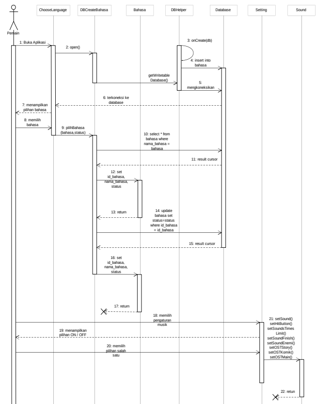
Gambar 3 Sequence Diagram
