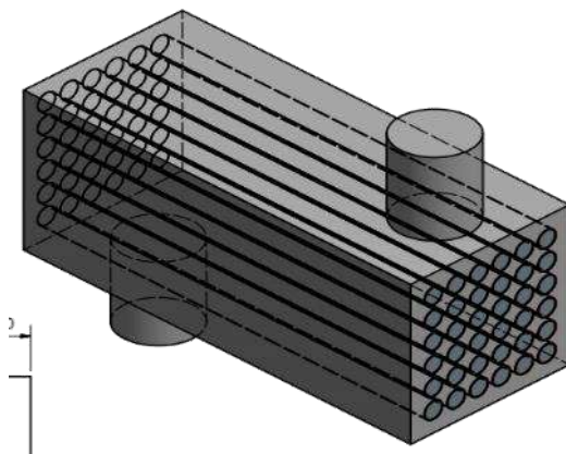
Gambar 2. Design alat penukar kalor
